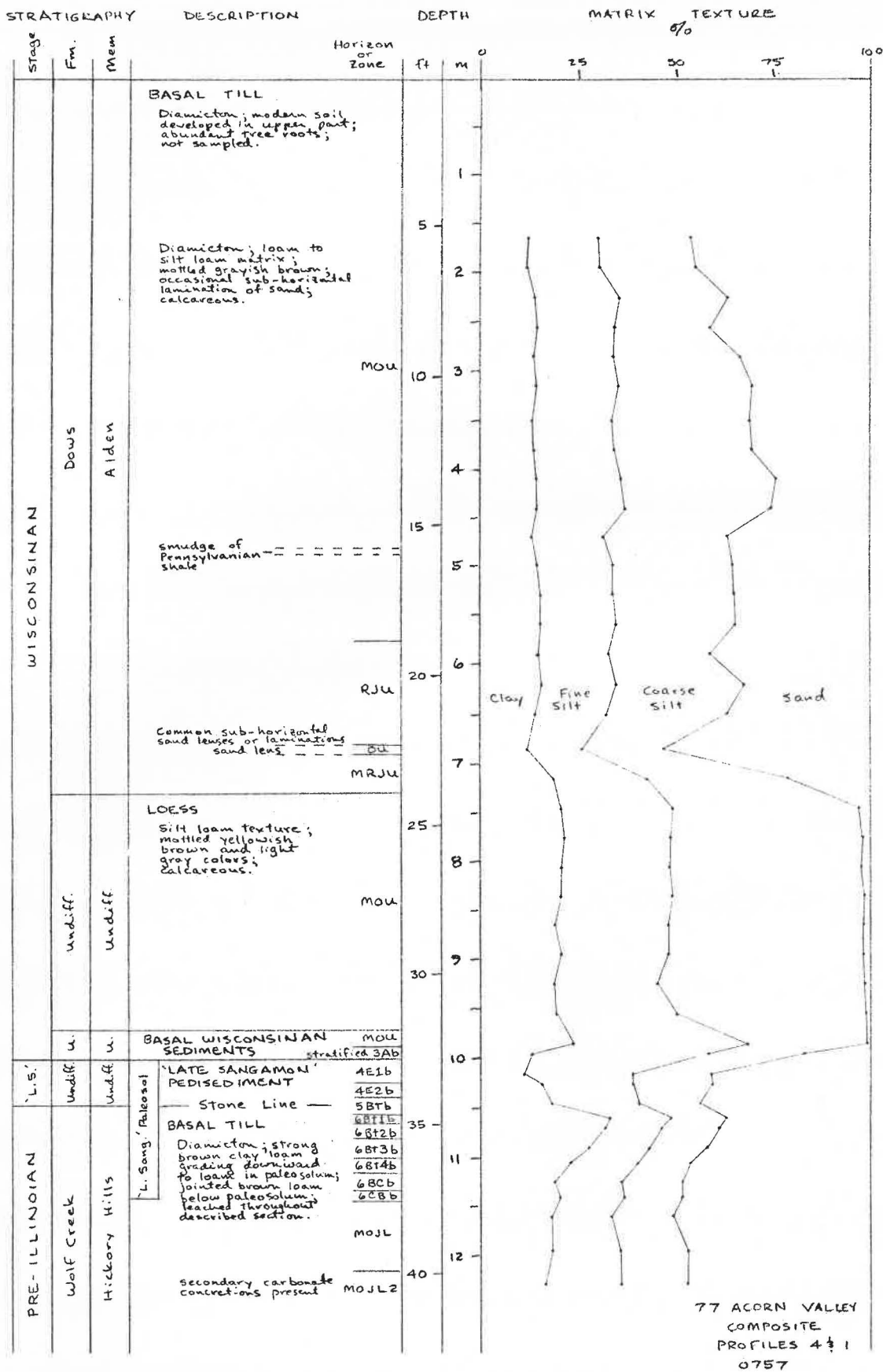
Figure 6-2. Stratigraphy and particle-size of profiles 4 and 1, Acorn Valley Section.
