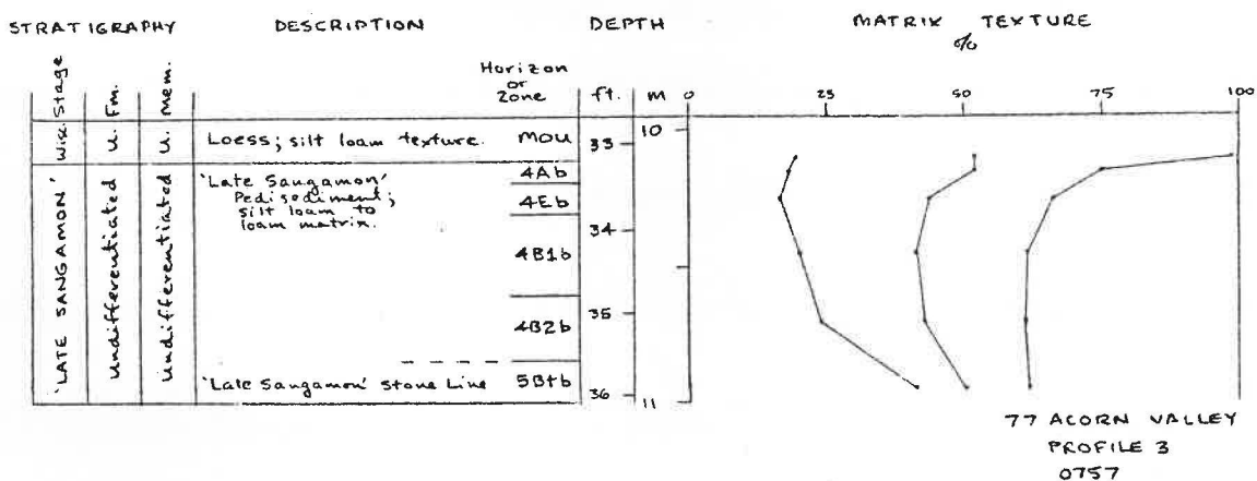
Figure 6-5. Stratigraphy and particle-size of profile 3, Acorn Valley Section. Only the 'Late Sangamon' pedisegment and stone line material was exposed and sampled.
