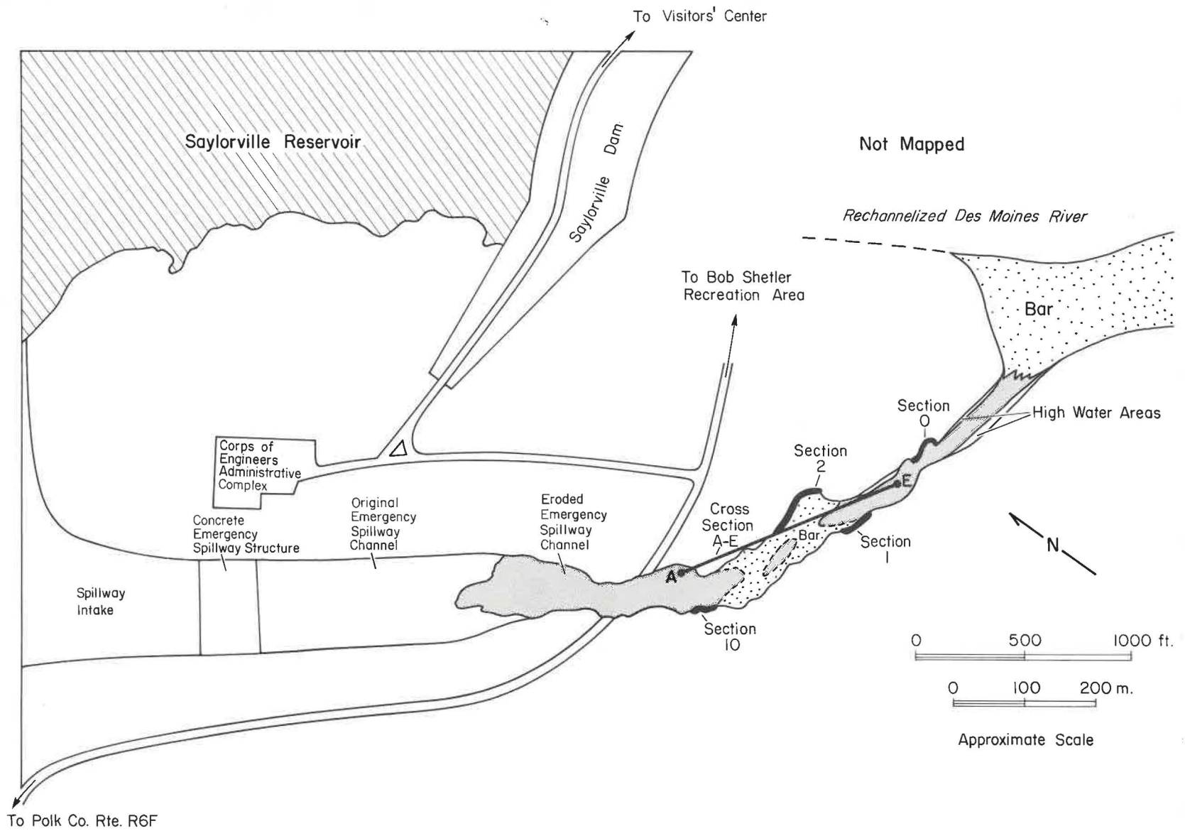
Figure 2-1. Sketch map of the Saylorville Emergency Spillway area.
