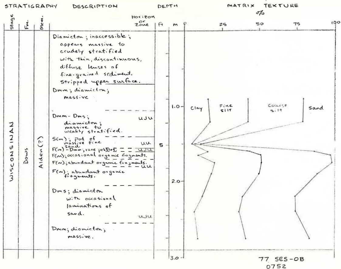
Figure 2-8. Stratigraphy and particle-size of profile B, Section 0. Profile location shown on Fig. 2-6.
