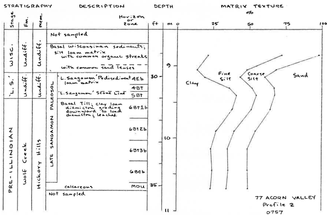
Figure 6-4. Stratigraphy and particle-size of profile 2, Acorn Valley Section.
