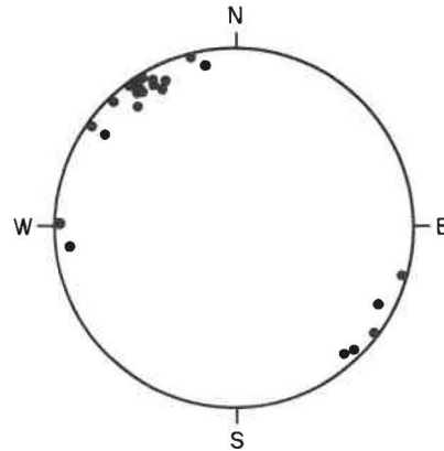
Figure 6-3. Fabric data for sites 1 and 2 in late Wisconsinan-age Des Moines Lobe diamicton at the Acorn Valley Section. Twenty-five prolate-shaped pebbles were measured for each. On the left data are plotted on lower hemisphere, Schmidt equal-area projections. On the right contoured equal area-projections (contoured according to the method of Kamb, 1959) are shown; contour interval = 2\sigma . Statistical orientation data calculated by the eigenvector method (Mark, 1973) are also shown.
