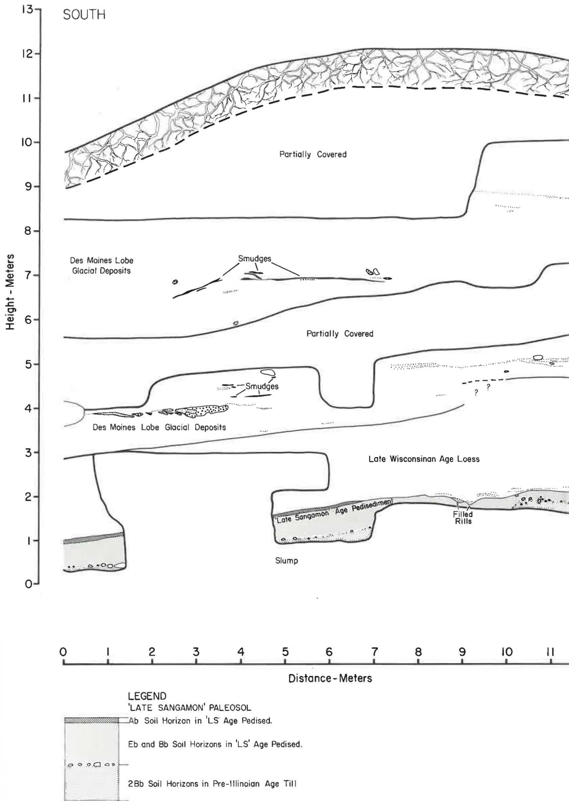
Figure 6-1. Detailed cross-section of the exposure of the Acorn Valley Section.
