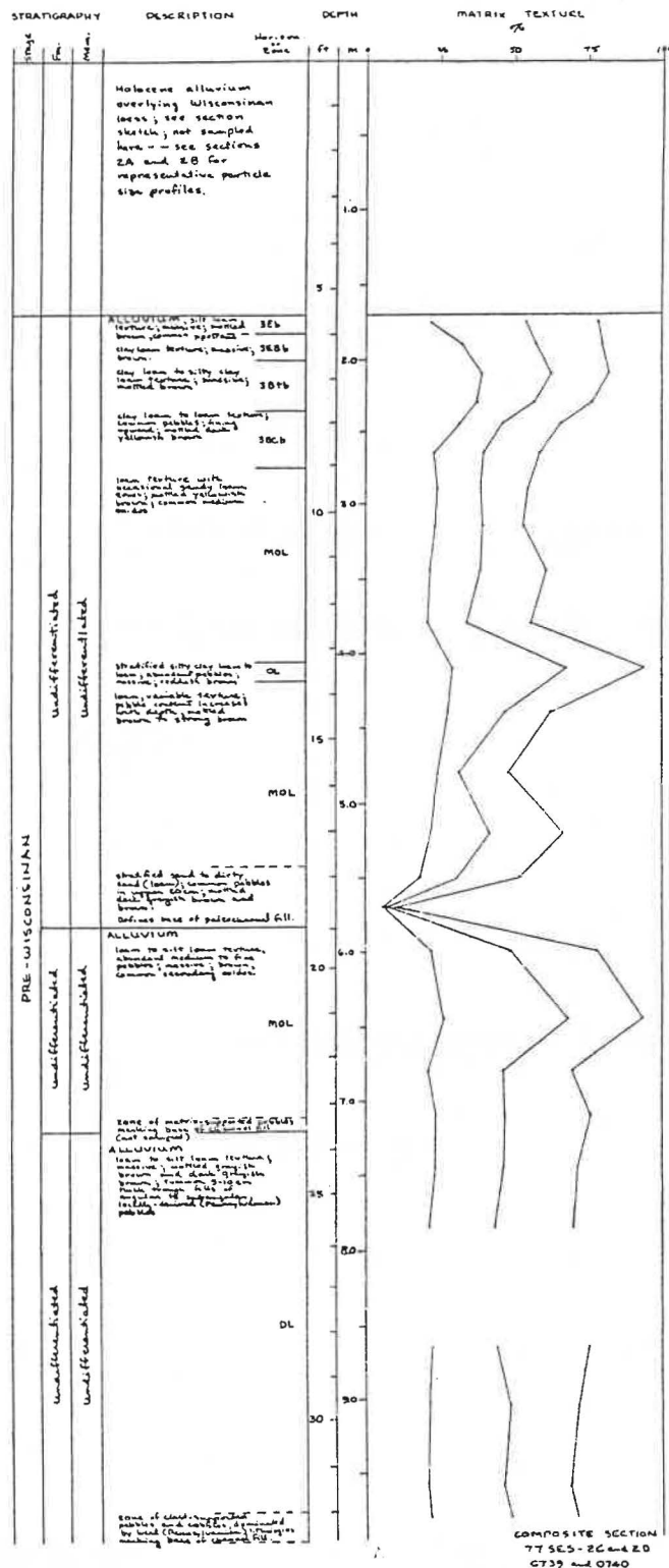
Figure 2-5. Stratigraphy and particle-size of profiles C and D, Section 2. Location of profiles shown on Fig. 2-3. 2-10
