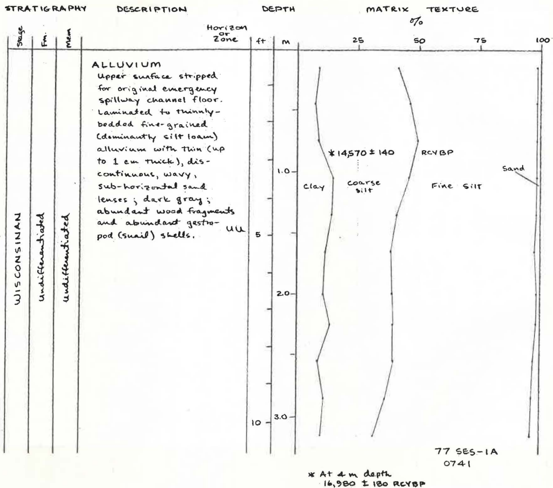
Figure 2-13. Stratigraphy and particle-size of profile A, Section 1. Profile location shown on Fig. 2-12.
