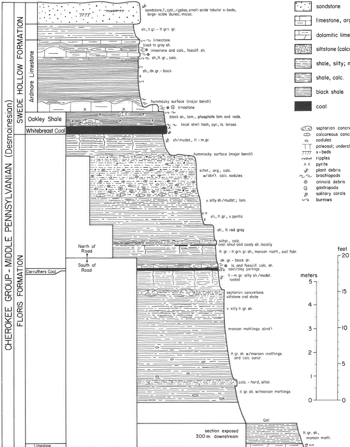
Figure 1-2. Stratigraphic sequence of Pennsylvanian deposits, Saylorville Canyon.
